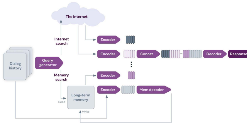
FIGURE 9. Facebook Chabot Blender bot 2.0, which utilize memorization and internet, search results [286].
