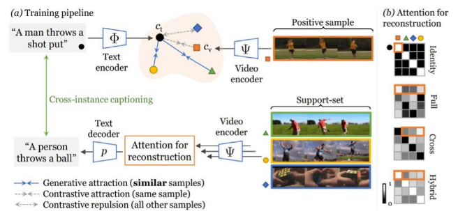
FIGURE 10. Multimodal training with videotext representation learning [296].
