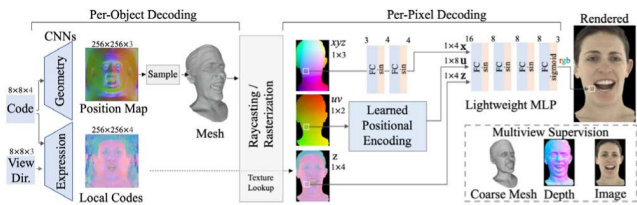
FIGURE 13. Face rendering with per-object decoding and per-pixel decoding in Pixel Codec Avatar [310].
