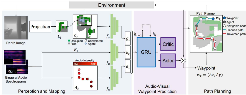
FIGURE 11. Learning to set waypoints for audio-visual navigation in the indoor environment [301].
